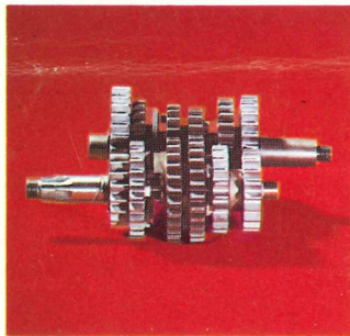
Over-sized 6-speed gearbox with undercut dogs.
