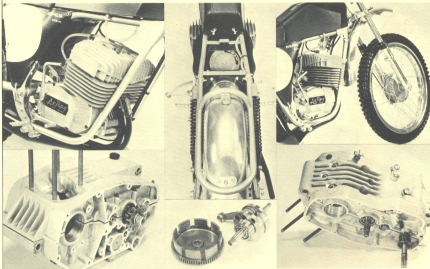
24 Horsepower/11:1 Compression ASPES CROSS 125 CC
